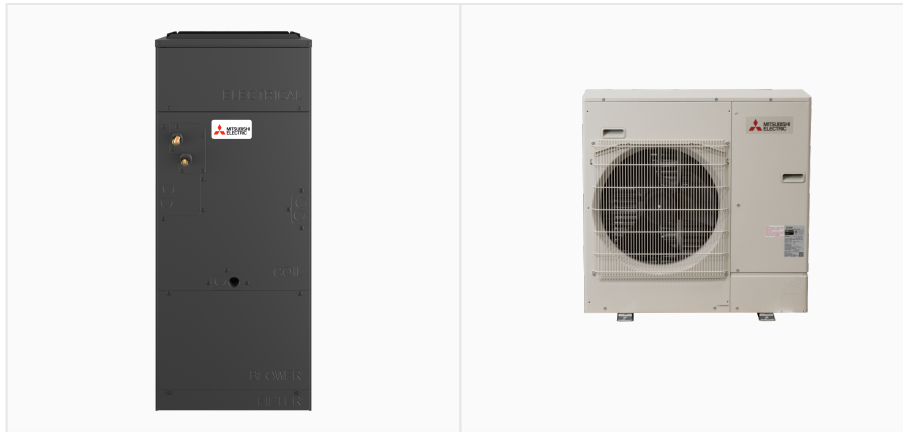
INDOOR Unit ... PVA-AA30NL OUTDOOR Unit ... PUY-AH30NL
