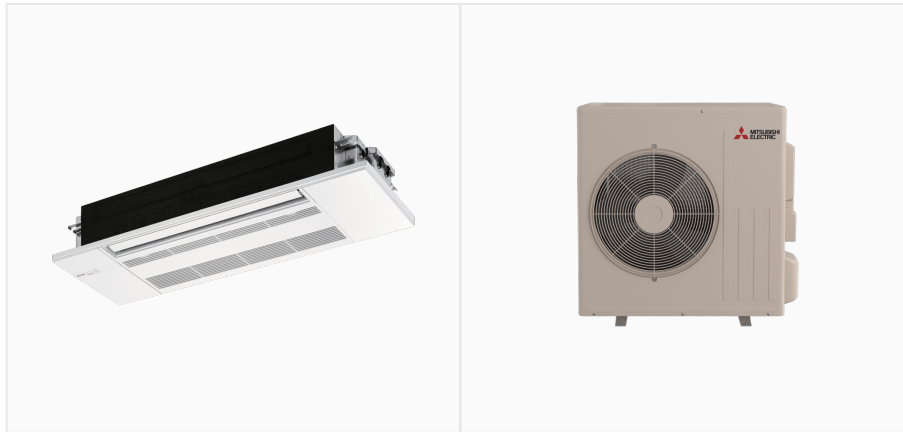
INDOOR Unit ... MLZ-KX18NL OUTDOOR Unit ... SUZ-AA18NL
